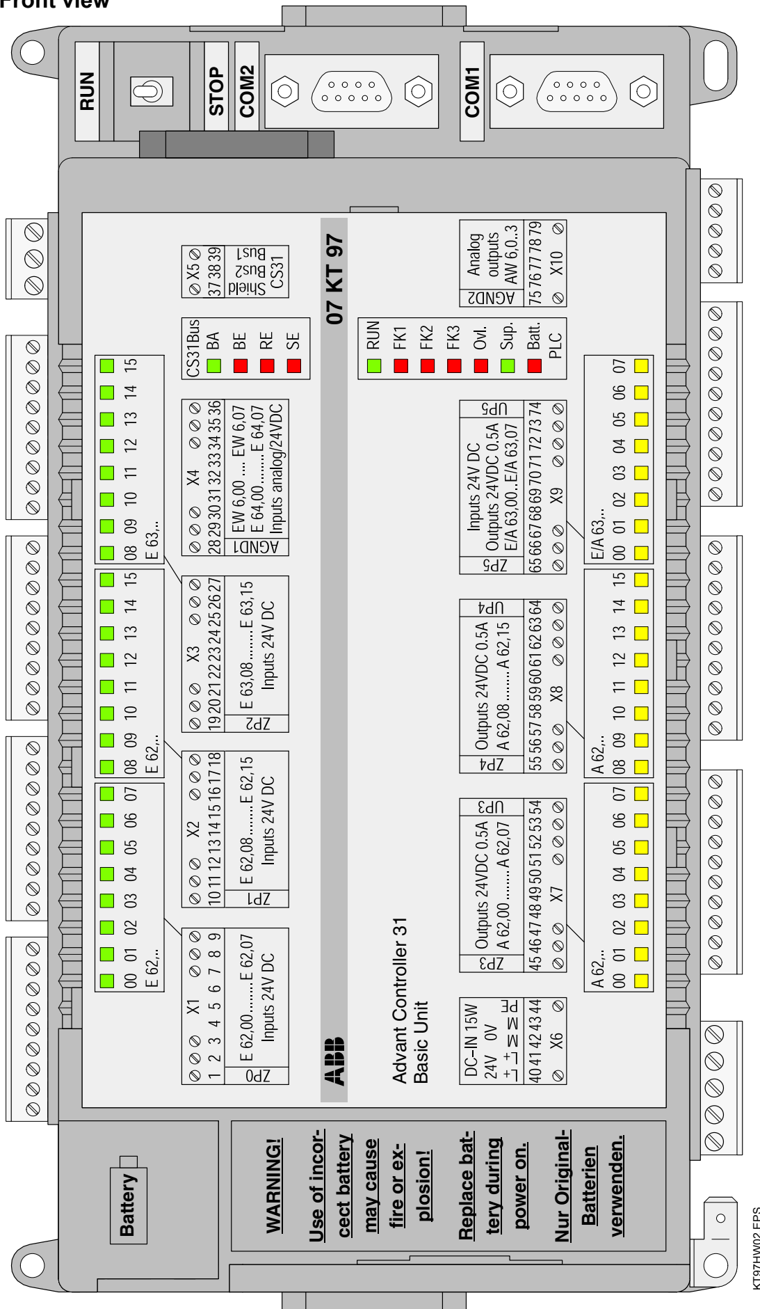
Fig. 2.1-2: Front view 07 KT 97 R200
