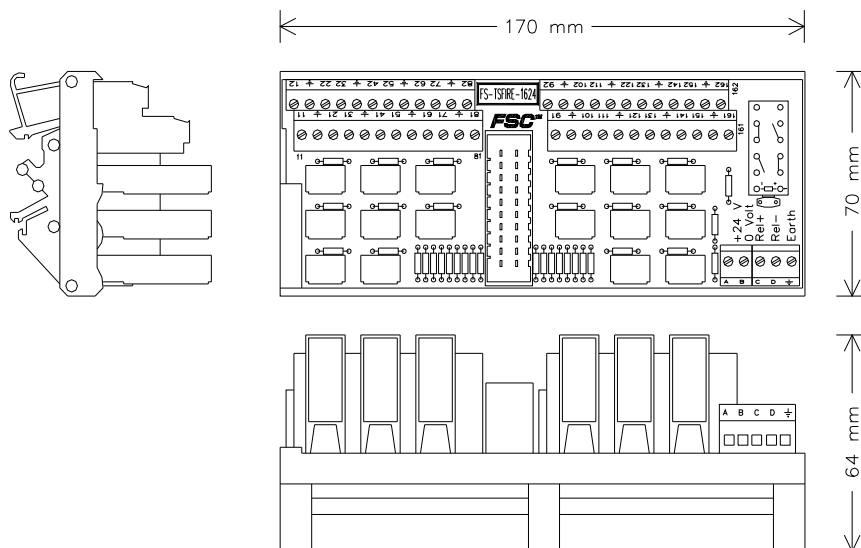
Figure 342 Mechanical layout
