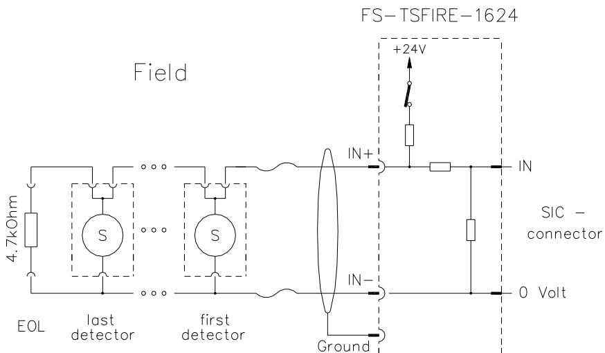
Figure 343 Typical schematic diagram for TSFIRE-1624 input
