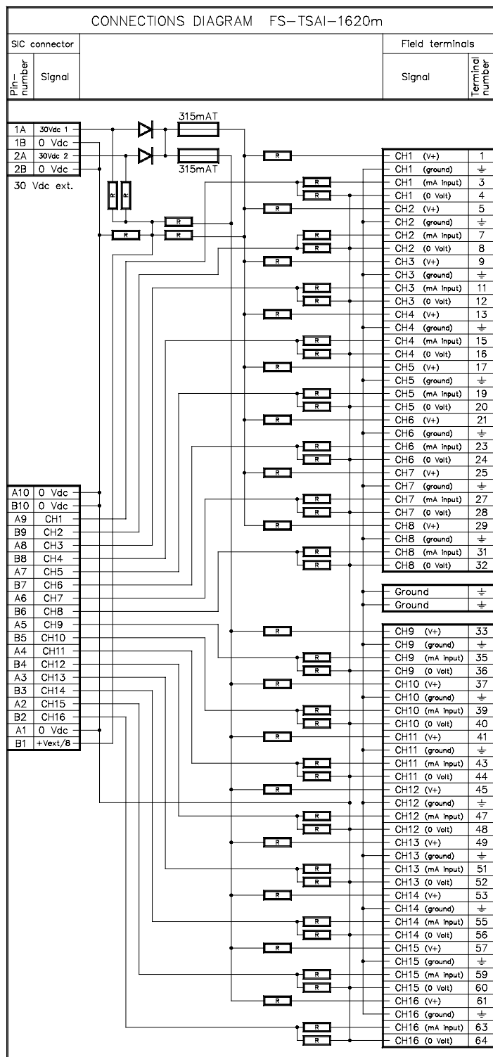
Figure 5 Connections diagram
