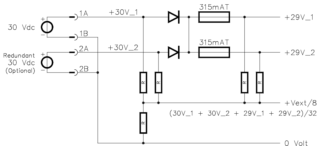
Figure 4 Schematic diagram for power distribution with monitoring
