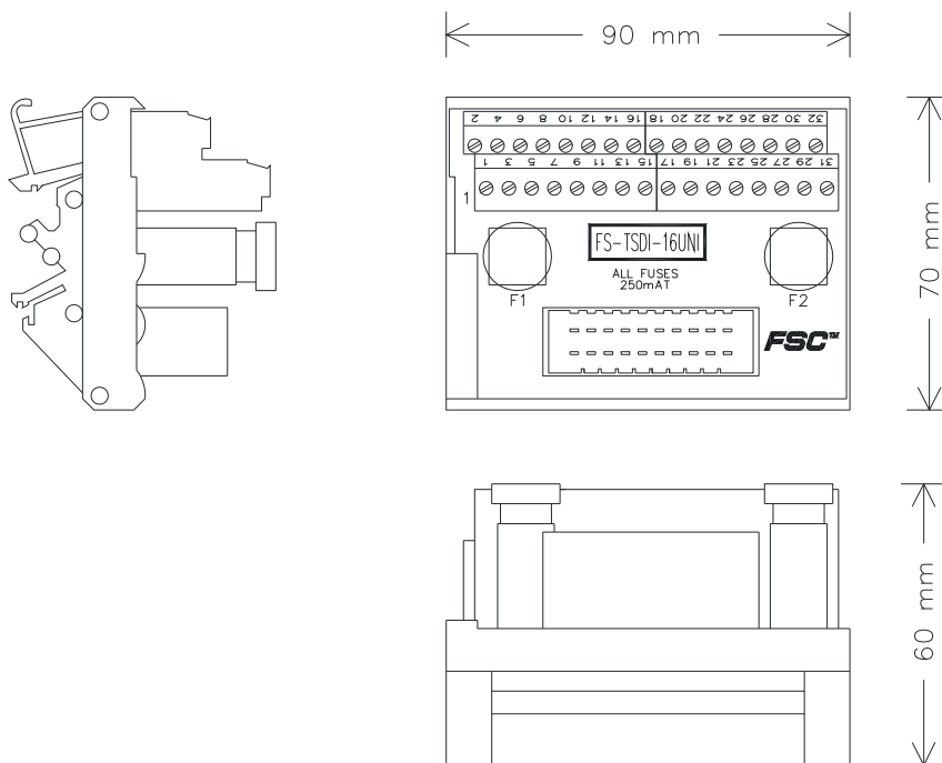
Figure 304 Mechanical layout
