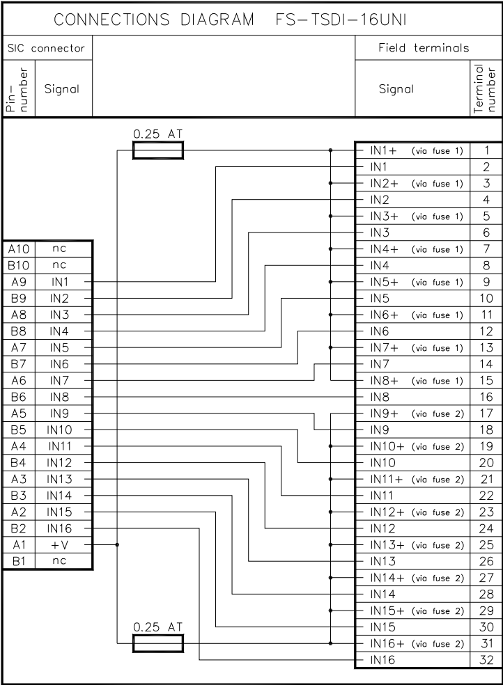
Figure 305 Connections diagram
