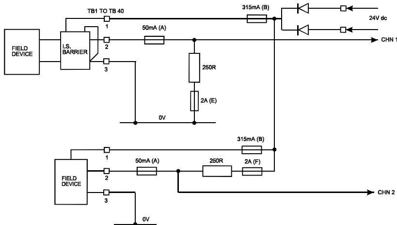
Single Channel Schematic for Current Sinking Gas Inputs
