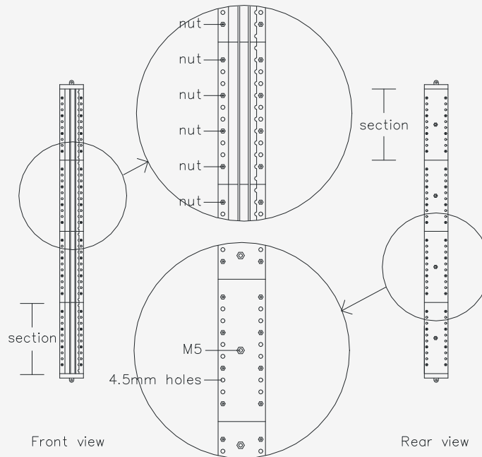
Figure 18-19: MB-0002 – 4 section power rail, front view and rear view
