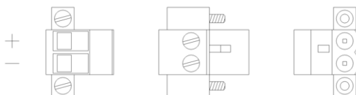
Figure 502 Power connector on Outx (Weidmuller BLZ 5.08/2F SN SW) top, side and bottom view
