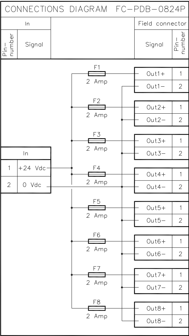
Figure 503 Connection diagram
