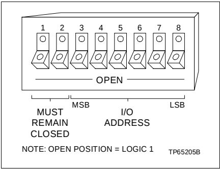
Figure C-2. Address Select Switch (S1)
