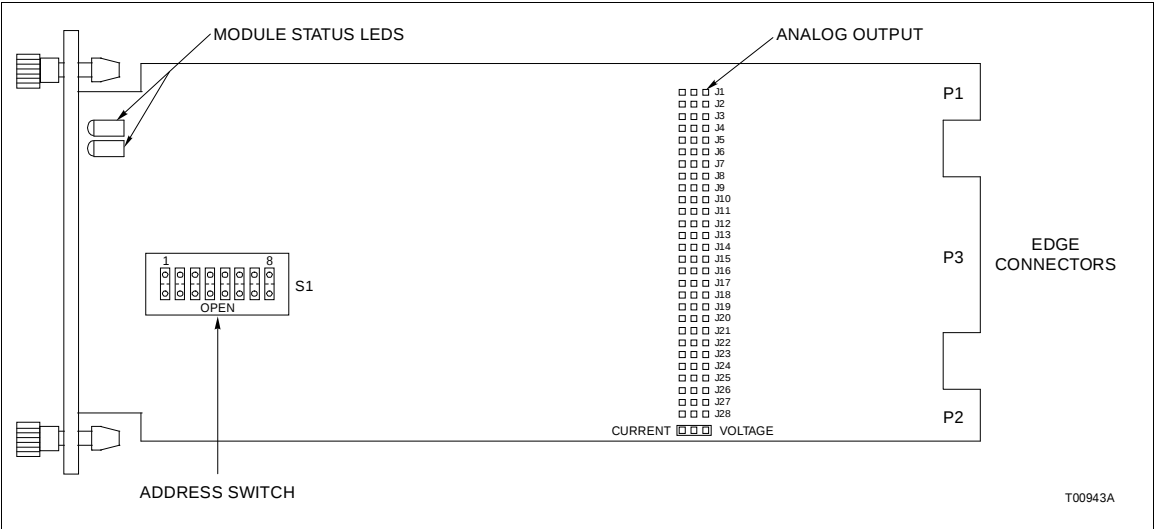
Figure C-1. Switch and Jumper Locations
