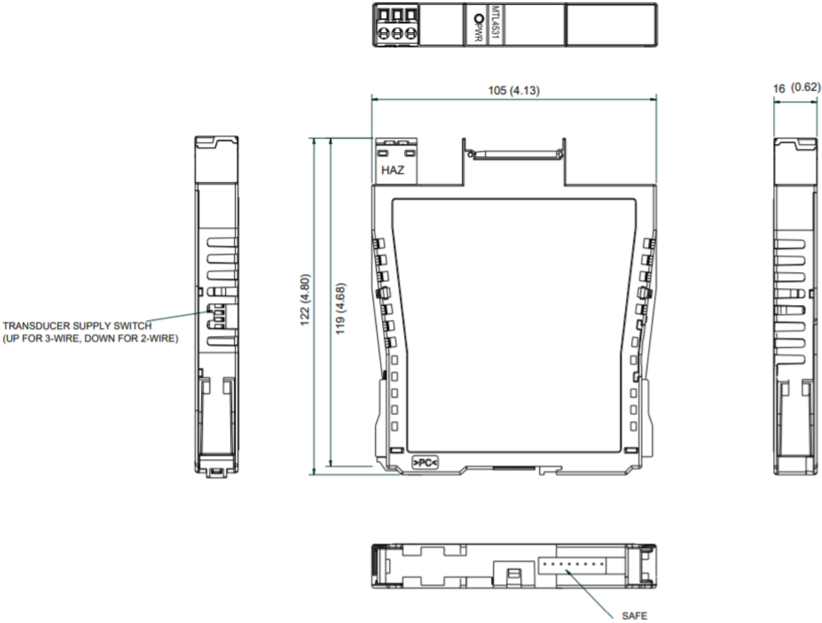
Figure 1: Dimensions of the MTL Vibration Galvanic Isolator Module, 288112
