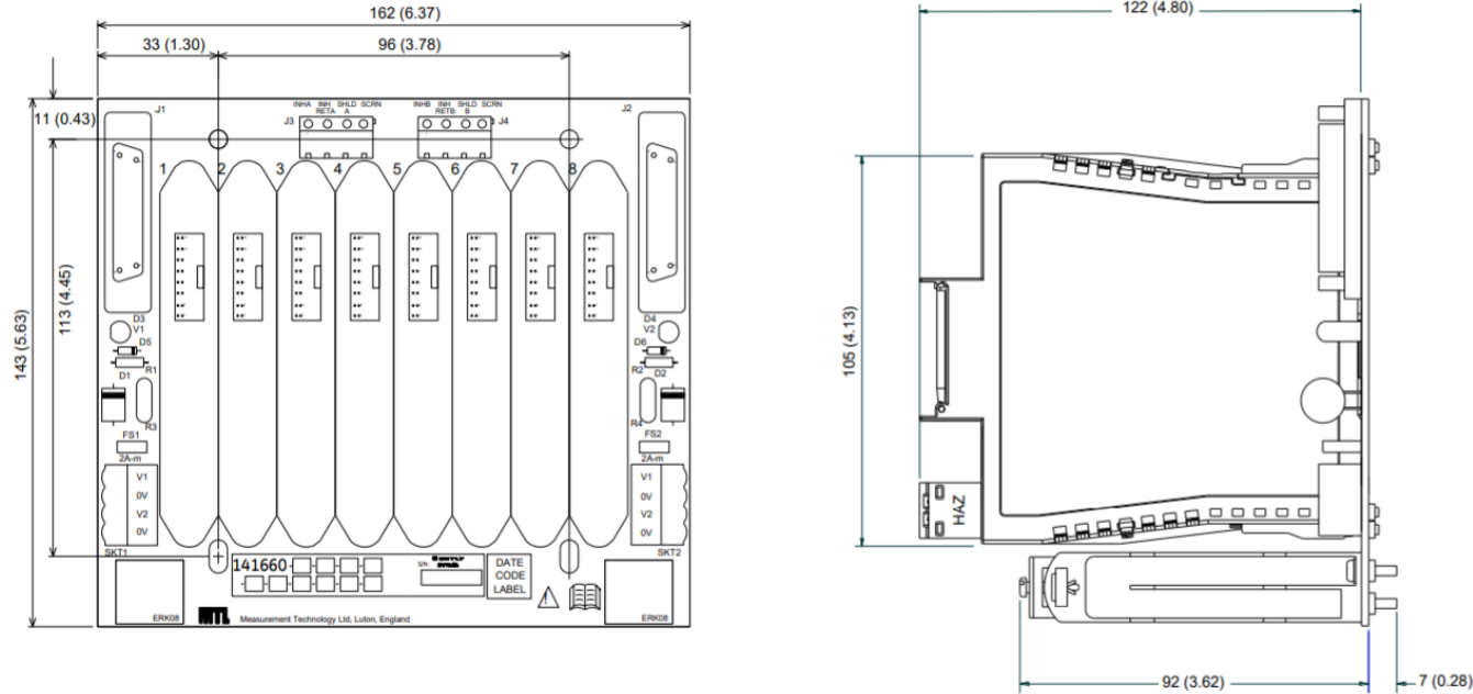
Figure 2: Dimensions of the MTL 8P Backplane, Vibration (288126)
