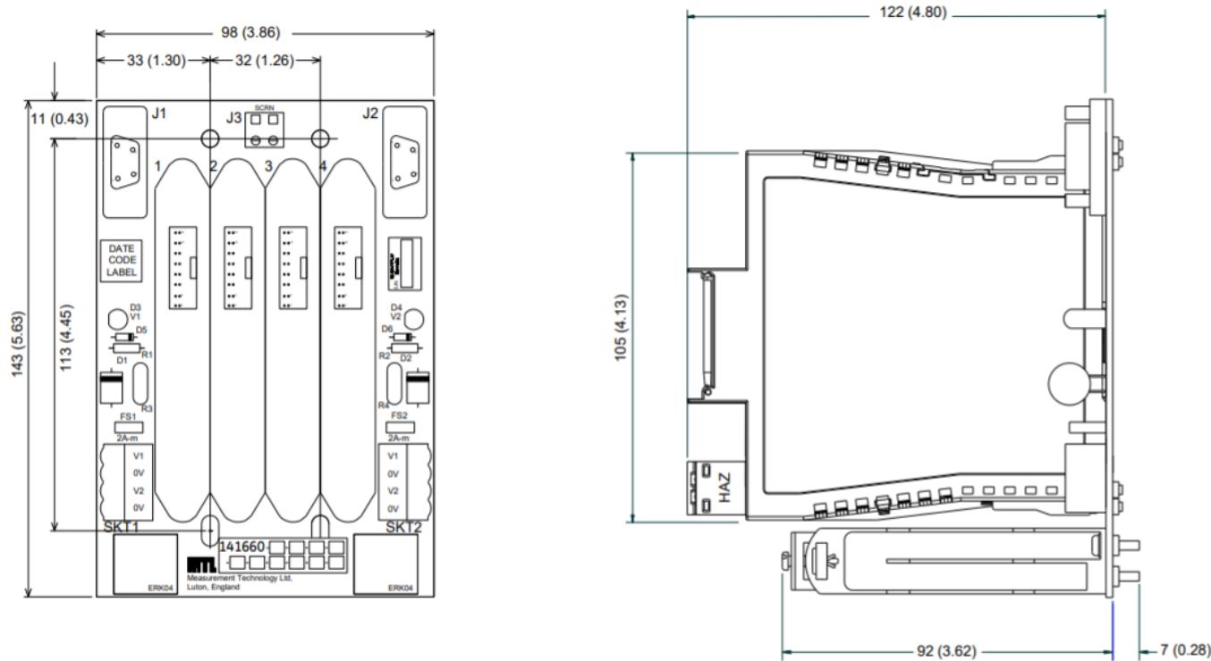
Figure 2: Dimensions of the MTL 8P Backplane, Vibration (288126)
